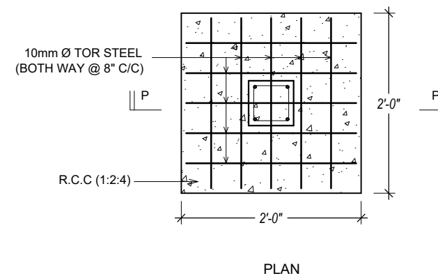
DETAIL OF SHORT COLUMNS DETAIL "C" SCALE : 1" = 2'-0"
