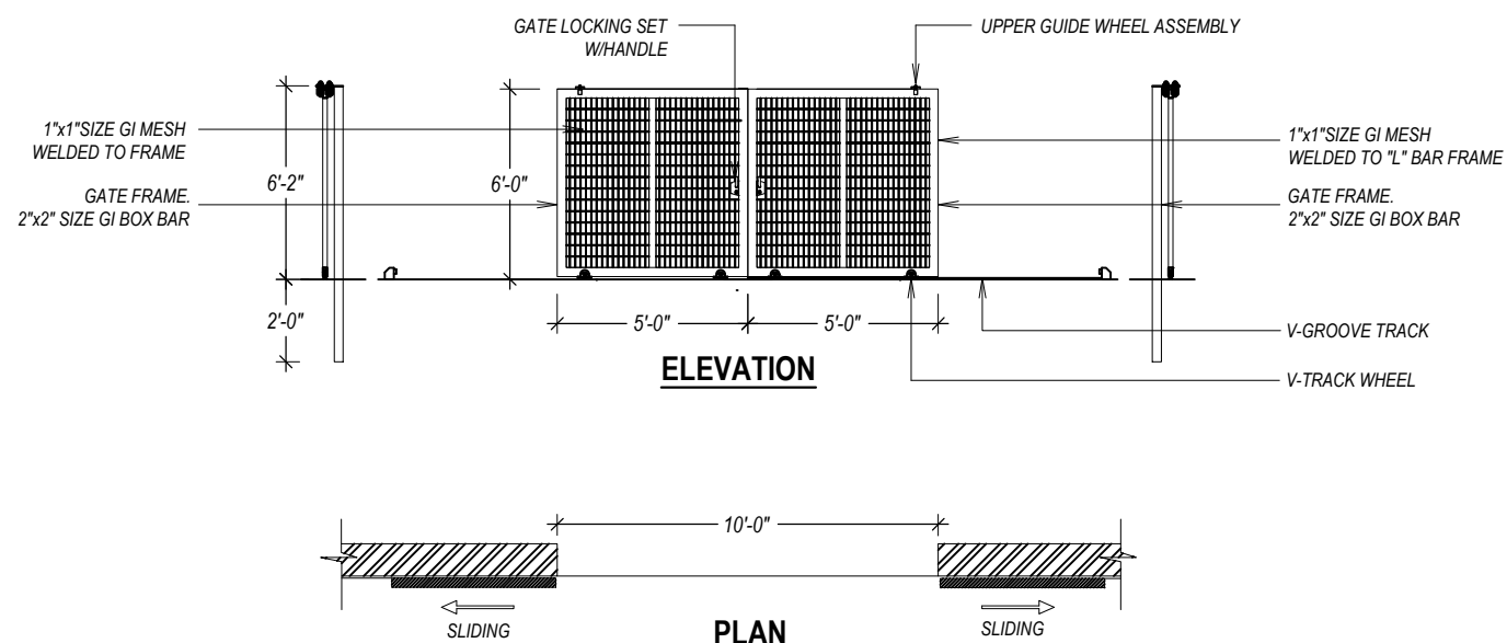
DETAILS OF STEEL GATE FRAME AND SASH
