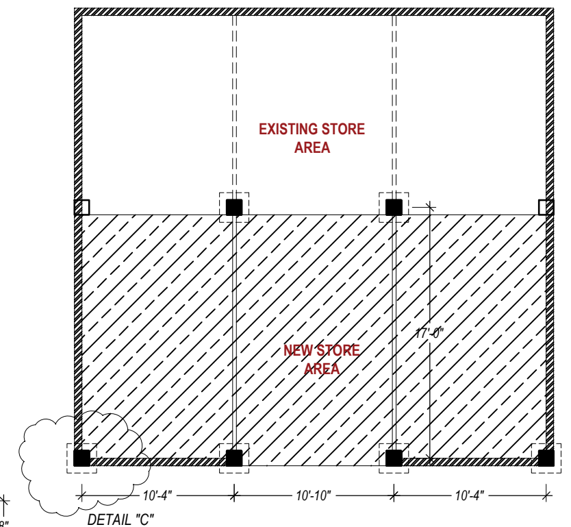
DETAILS OF COLUMN BASE AND STEEL COLUMNS
